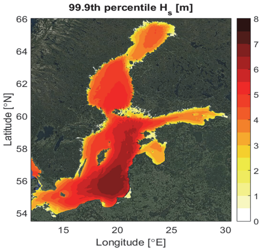
Fig. 3: Ice-free statistics (Type F in Tuomi et al. (2011)) for the 99.9 th percentile significant wave height using a high-resolution wave hindcast for the years 1998-2013 (Nilsson et al. 2019).
