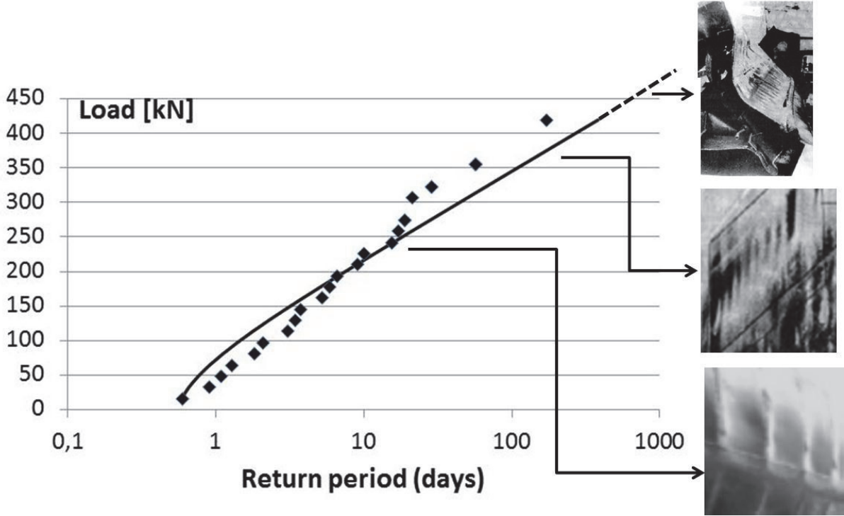
Figure 14. Measured load on one frame at the bow of MS Kemira measured during 1985-1991 (Kujala, 2017), showing also the possible effect of the increasing load on the damage of the ship shell structures.
